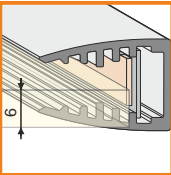
placement glass in the profile
