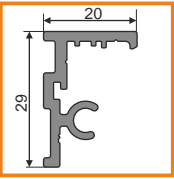
wall bracket SM
